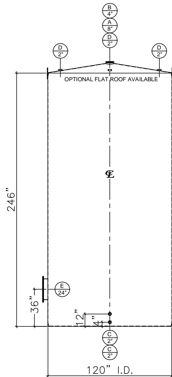
FRONT VIEW
